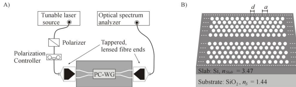
Fig. 1: (A) Experimental setup. (B) PC-WG configuration on a silicon-on-insulator (SOI) wafer comprising a SiO 2 layer and a silicon layer slab with an artificial periodicity of air holes.
